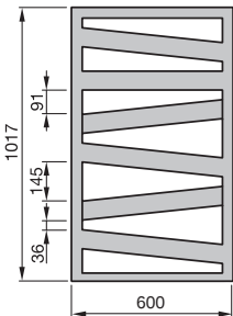
Front view RB(C)-100-600
