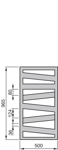
Front view RB(C)-100-500
