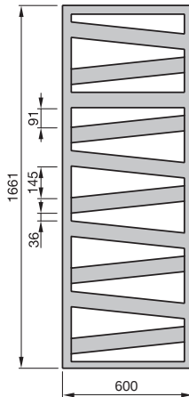
Front view RB(C)-170-600
