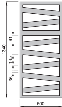
Front view RB(C)-130-600
