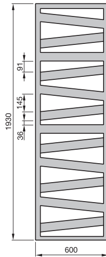
Front view RB(C)-190-600
