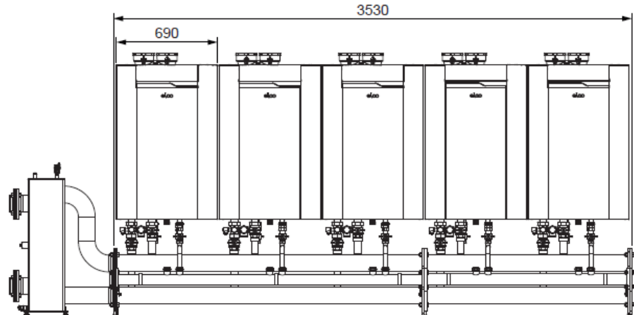
THISION L PLUS 5 boilers wall mounted in line
