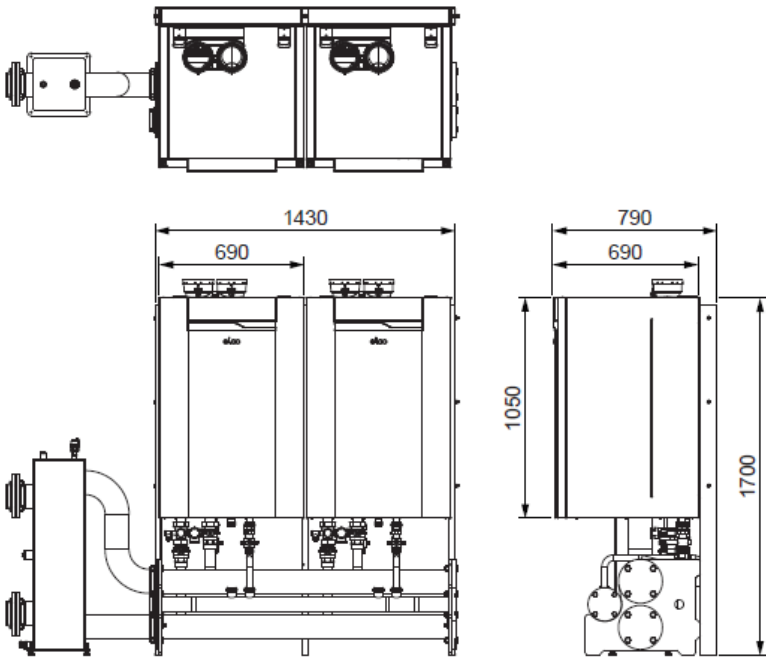
THISION L PLUS 3 boilers free-standing in line
