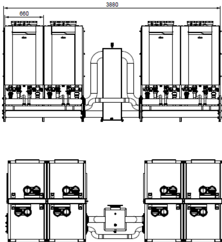
THISION L PLUS 8 boilers free-standing back-to-back
