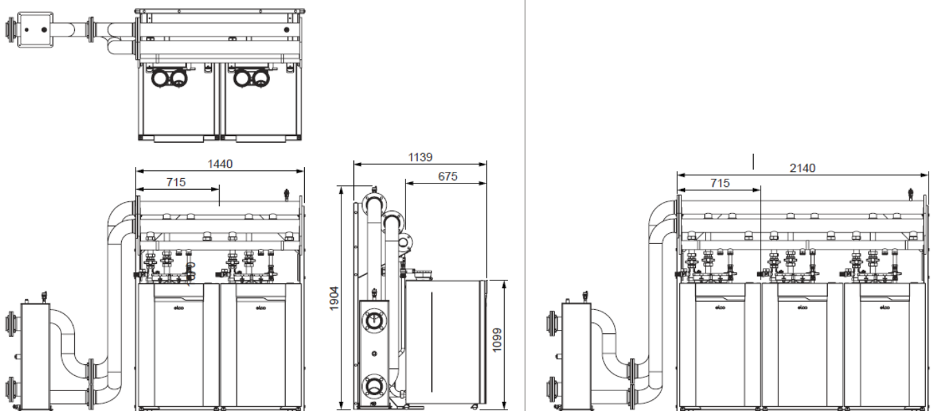
TRIGON L PLUS 2 boilers floor standing in line
