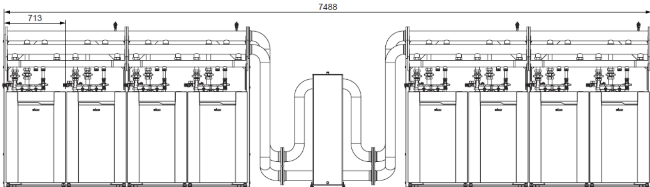
TRIGON L PLUS 8 boilers floor standing in line
